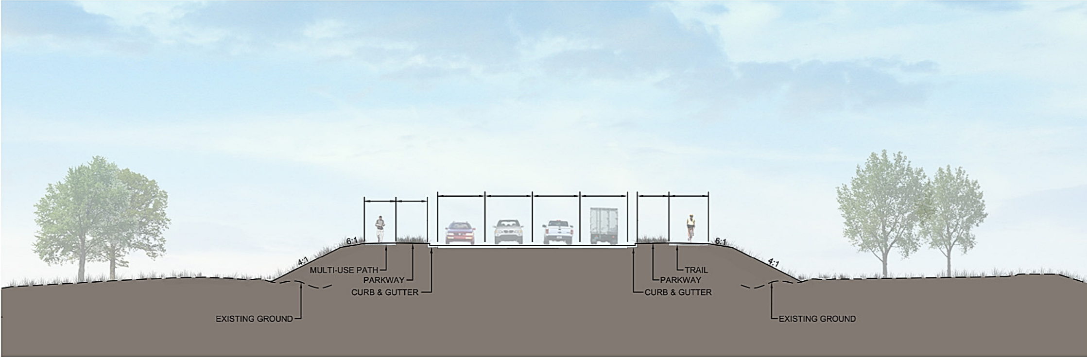
Typical Section Curb and Gutter, No Median
