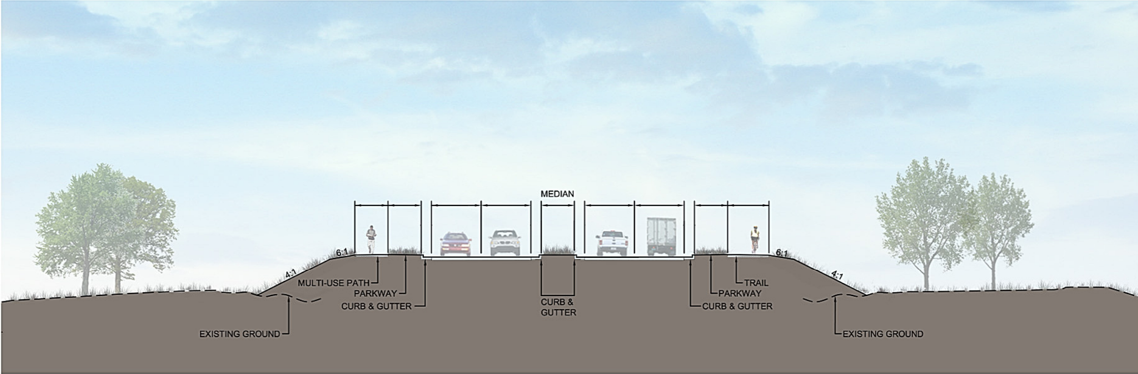
Typical Section Curb and Gutter with Median
