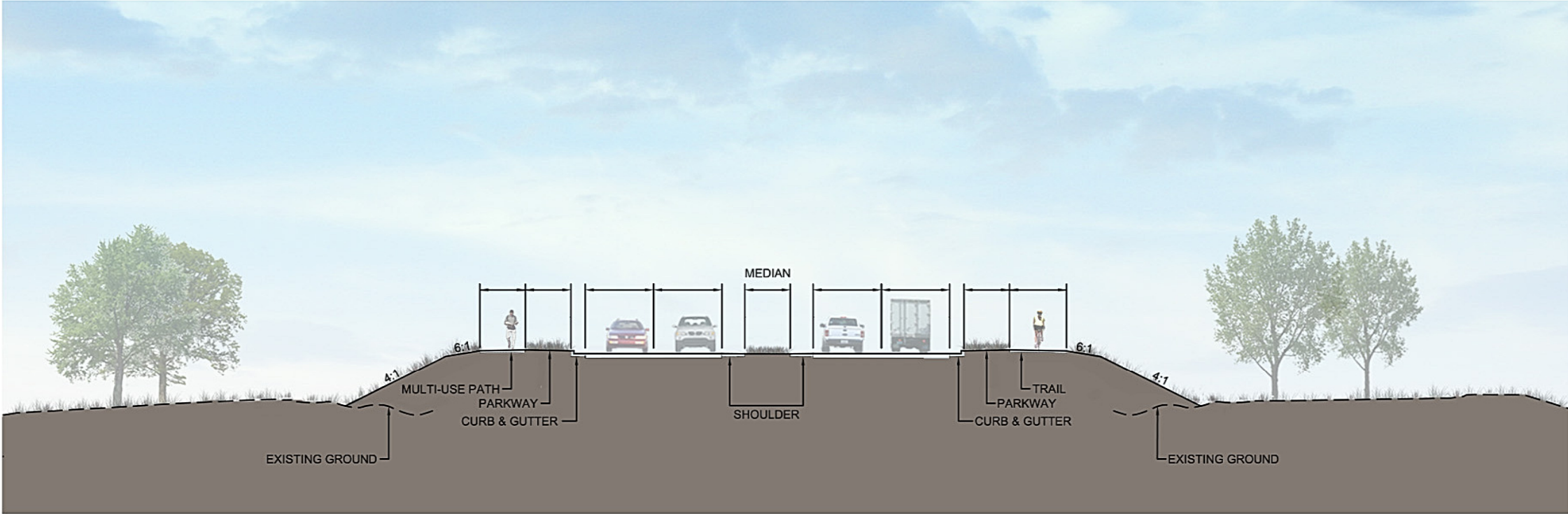
Typical Section Rural Median
