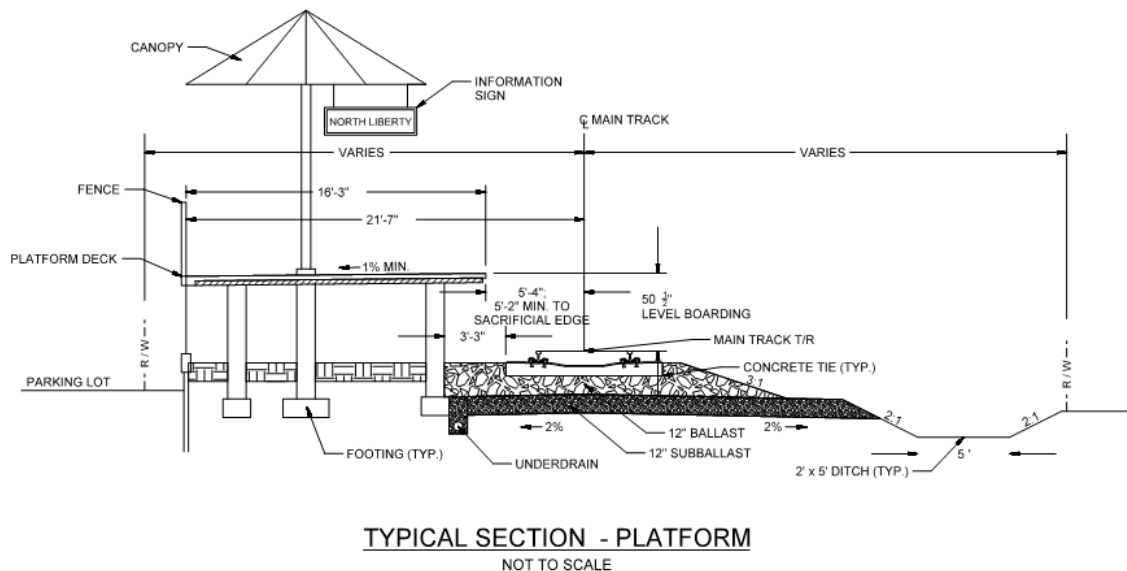
Figure 19: Typical Station Platform Concept
